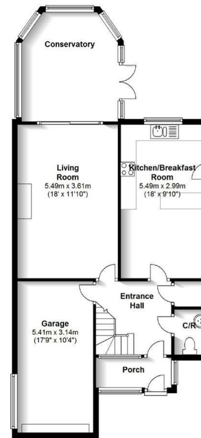
Ground Floor Approx. 87.9 sq. metres (946.7 sq. feet)
